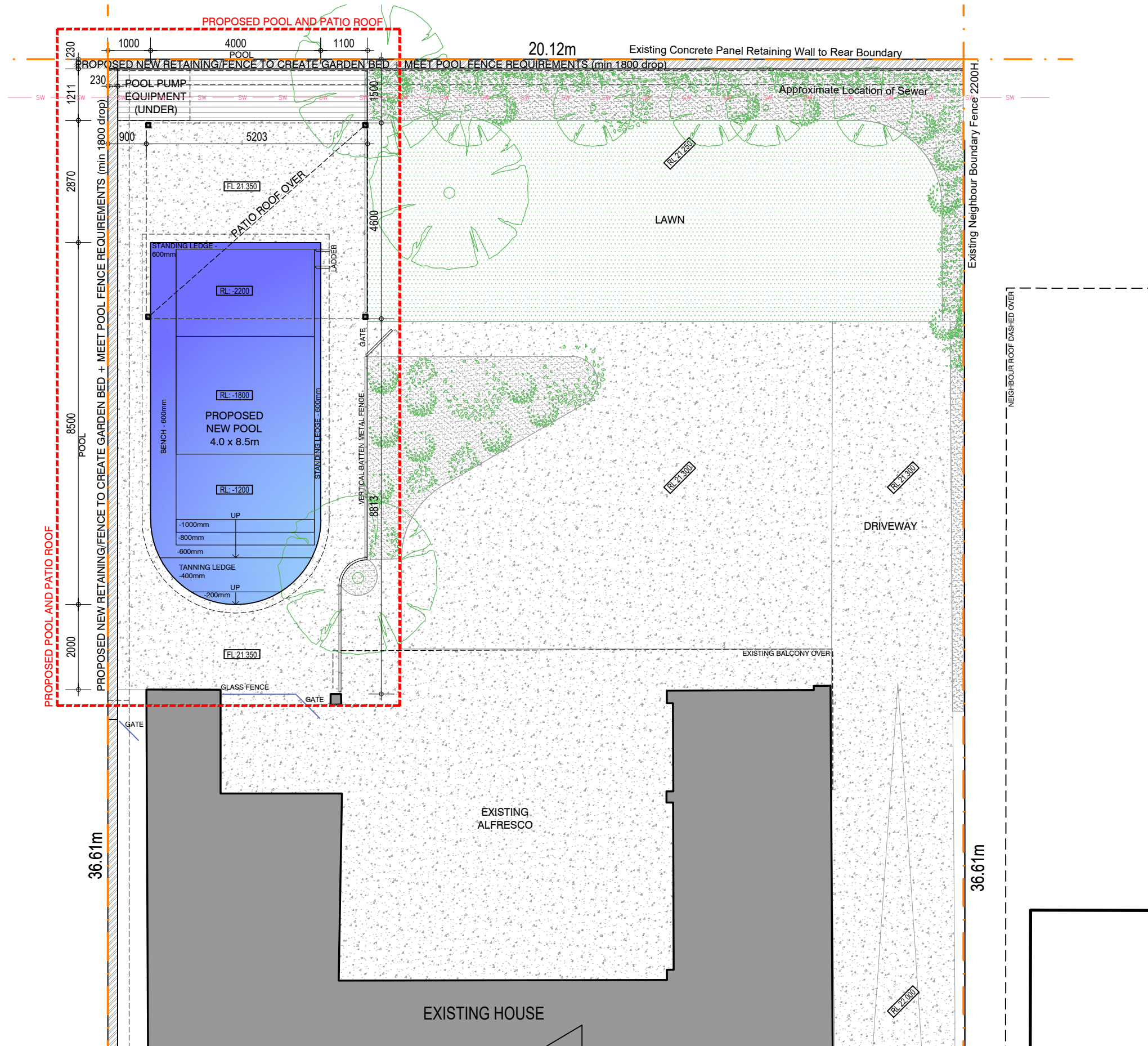
1 PLAN - POOL 1:100
